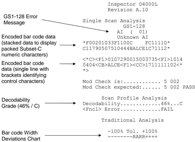
Figure I-1 (GS1-128 Failure)
