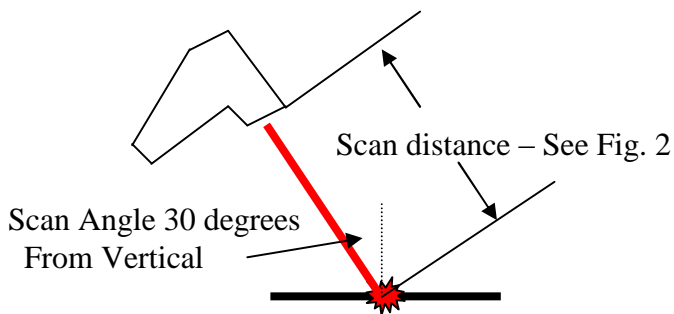
Figure 2 – Optimum beam width and placement
